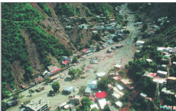
Large volume of sediments, rudiments of buildings and other debris were transported by debris flows and high flood water
